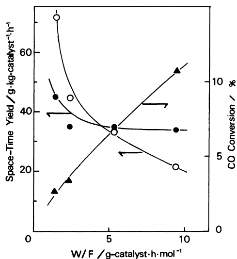
Fig. 3. Effect of time factor on CO conversion (▲) and space-time yields of alcohols (○) and hydrocarbons (●) over Mo(20 \text{ wt}\%) + KCl(K=1.63 \text{ wt}\%)/SiO_2(ID) catalyst at 573 K and 1.6 MPa.
