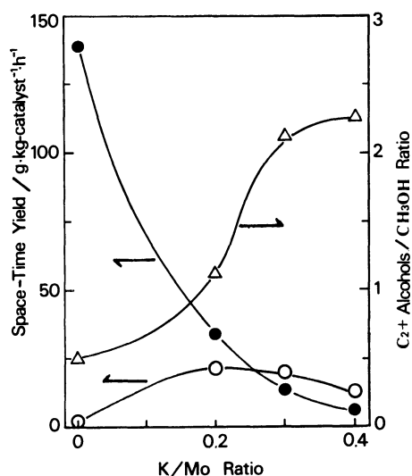
Fig. 1. Effect of K content (K/Mo ratio) on space-time yields of alcohols (○) and hydrocarbons (●), and C_2+OH/CH_3OH ratio (△) over Mo(20 \text{ wt}\%) + KCl/SiO_2(ID) at W/F=10 \text{ g-catalyst h mol}^{-1} , 573 K, and 1.6 MPa.
